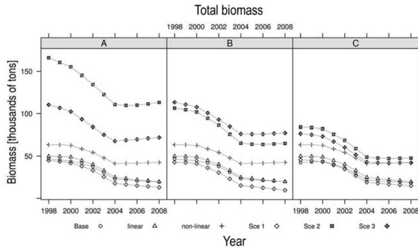
Figure 6. Total biomass comparison between age-structured and biomass dynamic model across cases (A, B, C) and scenarios.
