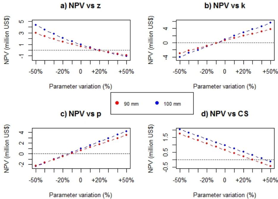
Figure 3. Expanded sensitivity analysis for Case 2: Independencia Bay after variations in a) mortality rate ( z ), b) growth parameter ( k ), c) price ( p ), d) seed cost ( CS ).
