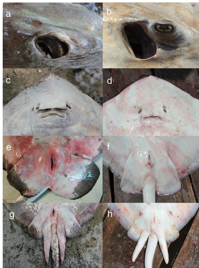
Figure 2. Morphological characteristic of eyeless and regular (normal) southern stingrays, Dasyatis americana , caught on the Campeche Bank (southern Gulf of Mexico). a) eyeless, and b) eye detail of a normal individual; nasal curtain of c) eyeless, and d) normal individual, pelvic fins of e) eyeless, and f) normal female; pelvic fins and claspers of g) eyeless, and h) normal males.
