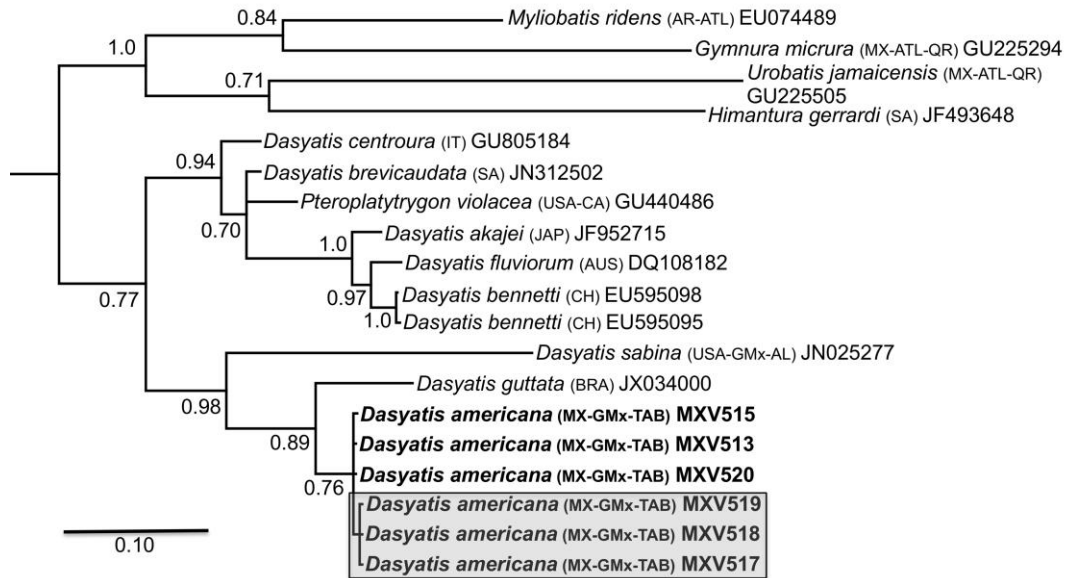
Figure 3. Bayesian majority-rule consensus phylogram of mitochondrial DNA Cytochrome Oxidase I (mt DNA COI) bar code gene of stingrays (Rajiformes). 650 bp of the mtDNA COI bar code gene were used. Support values on branches are Bayesian posterior probabilities. Sequences include species name from which it derives, followed by its geographic location and GenBank™ accession number. Sequences from Dasyatis americana are in bold font and sequences from eyeless D. americana are highlighted in the gray-shaded square. Sequences from Myliobatis ridens Ruocco, Lucifora, Díaz de Astarloa, Mabragaña & Delpiani, 2012 (Myliobatidae), Gymnura mycrura (Bloch & Schneider, 1801) (Gymnuridae), Himantura gerrardi (Gray, 1851) and Urobatis jamaicensis (Cuvier, 1816) (Urotrygonidae) were used as outgroups to root the phylogeny. AR: Argentina, MX: Mexico, SA: South Africa, IT: Italy, USA: United States of America, JAP: Japan, AUS: Australia, CH: China, BRA: Brazil, QR: Quintana Roo, CA: California, AL: Alabama, TAB: Tabasco, ATL: Atlantic Ocean, GMx: Gulf of Mexico. Scale indicates percentage sequence divergence among haplotypes.
