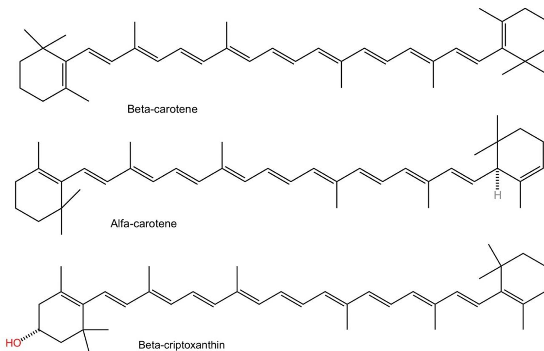
Figure 3. Chemical structure of carotenoids with the higher activity of provitamin A.
