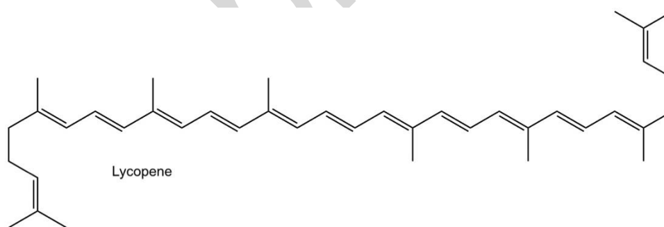
Figure 2. Chemical structure of lycopene, the prototypic molecule of carotenoids.
